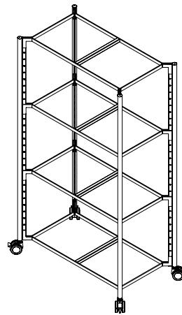
PIXEL RACK M 820x460,5x1478 mm
