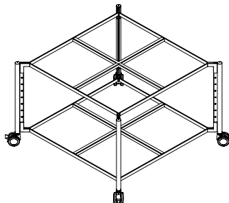
PIXEL RACK L 820x820x564 mm
