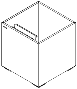
PIXEL BOX GESCHLOSSEN PIXEL BOX CLOSED 360x360x381 mm
