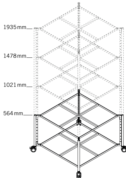
PIXEL RACK L 820x820 mm
