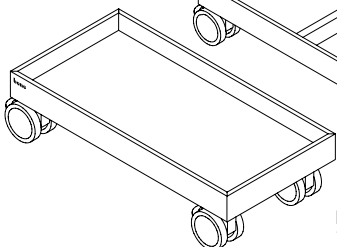
PIXEL TRAY 360x360x61 mm
